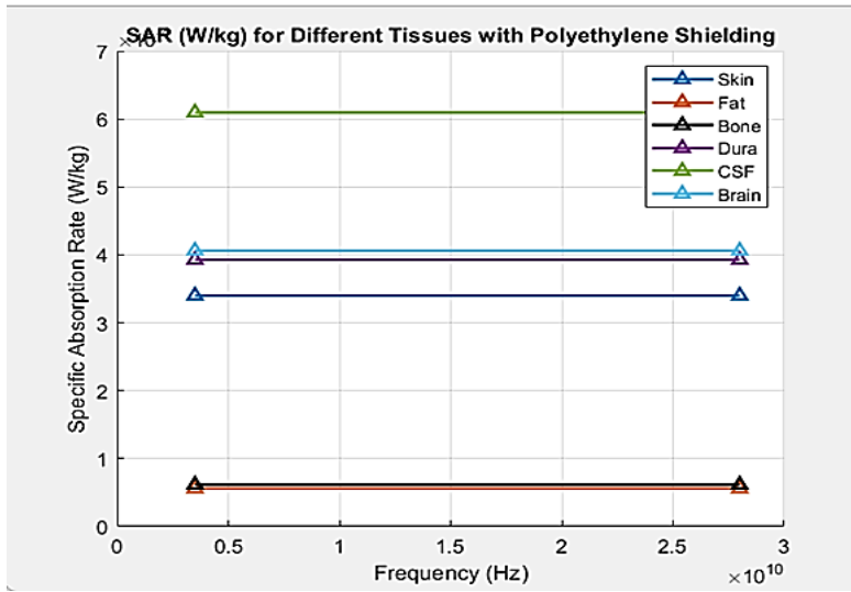
Figure 5. SAR (W/kg) (for tissues with Polyethylene shielding)
