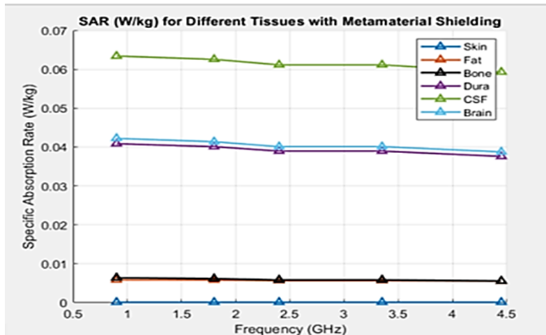
Figure 4. SAR (W/kg) for tissues with metamaterial shielding.
