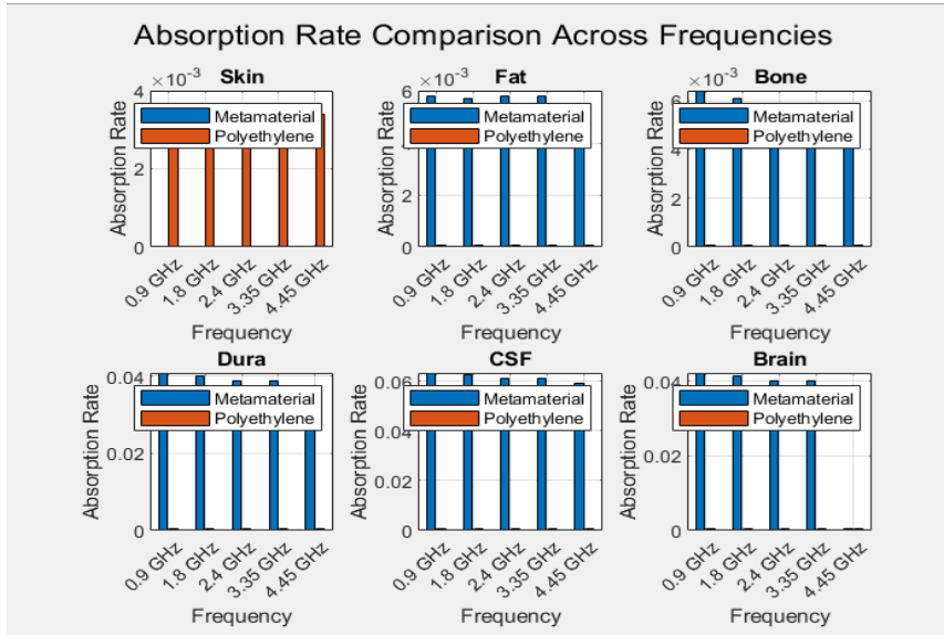
Figure 6. The specific absorption rate graph of Metamaterials and polyethylene
